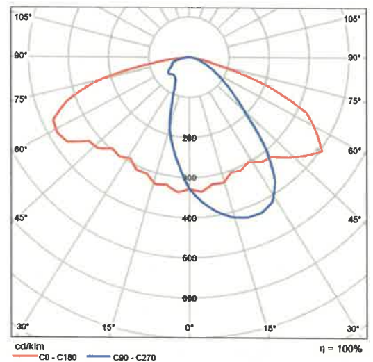
Polar LDC
