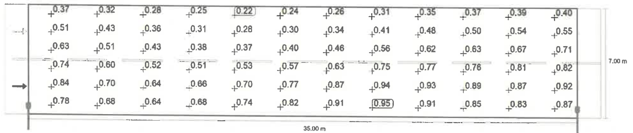
Observer 1: Luminance with new installation [cd/m²] (Value grid)
