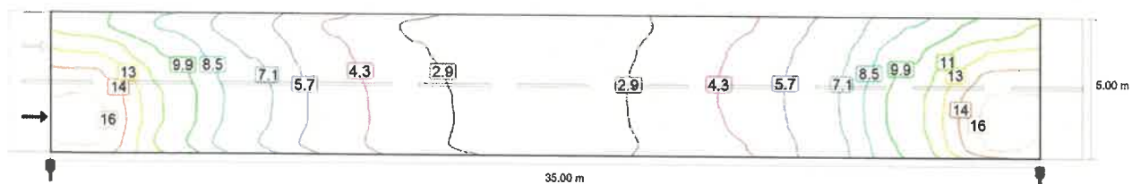
Maintenance value, horizontal illuminance [lx] (Iso-illuminance curves)
