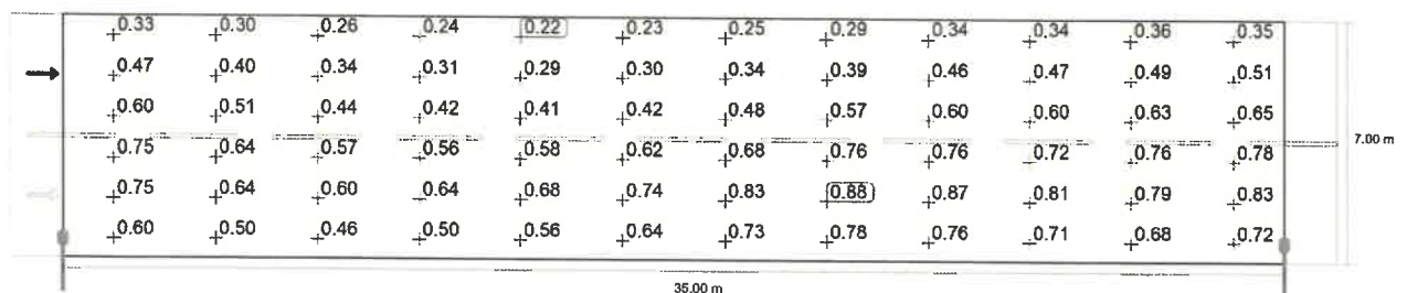
Observer 2: Maintenance value, luminance with dry roadway [cd/m²] (Iso-illuminance curves)
