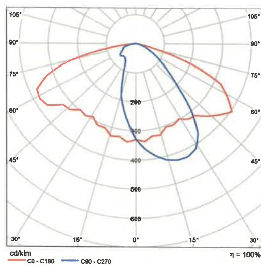
Polar LDC
